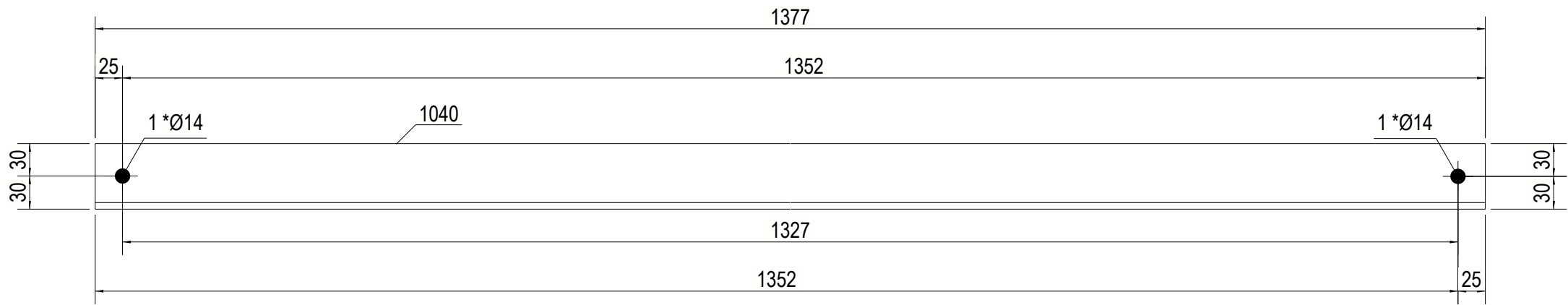
FRONT VIEW
